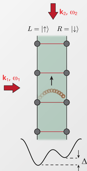
Spin-Momentum locking: D. Hügel, B. Paredes, PRA 89, 023619 (2014)
