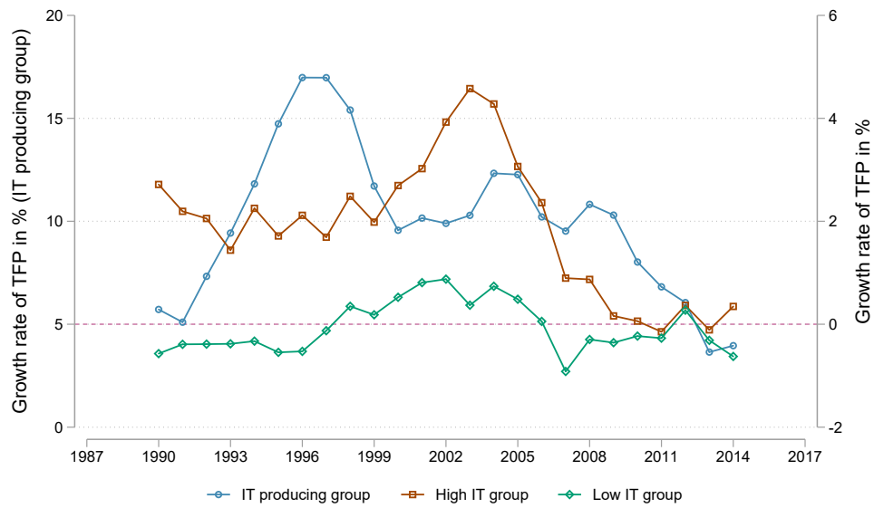
Figure E4: Productivity growth by IT intensity - Alternative 4
