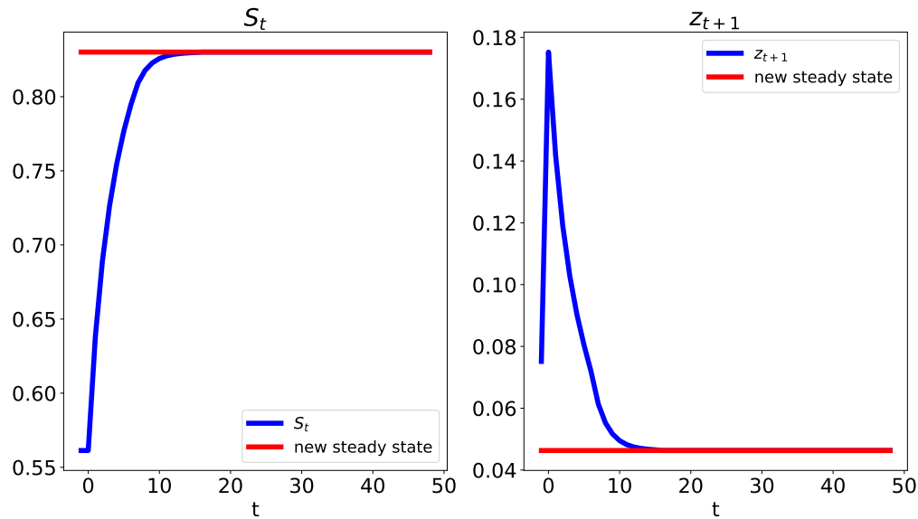
Figure 8: Transition dynamics of S_t and z_{t+1}
