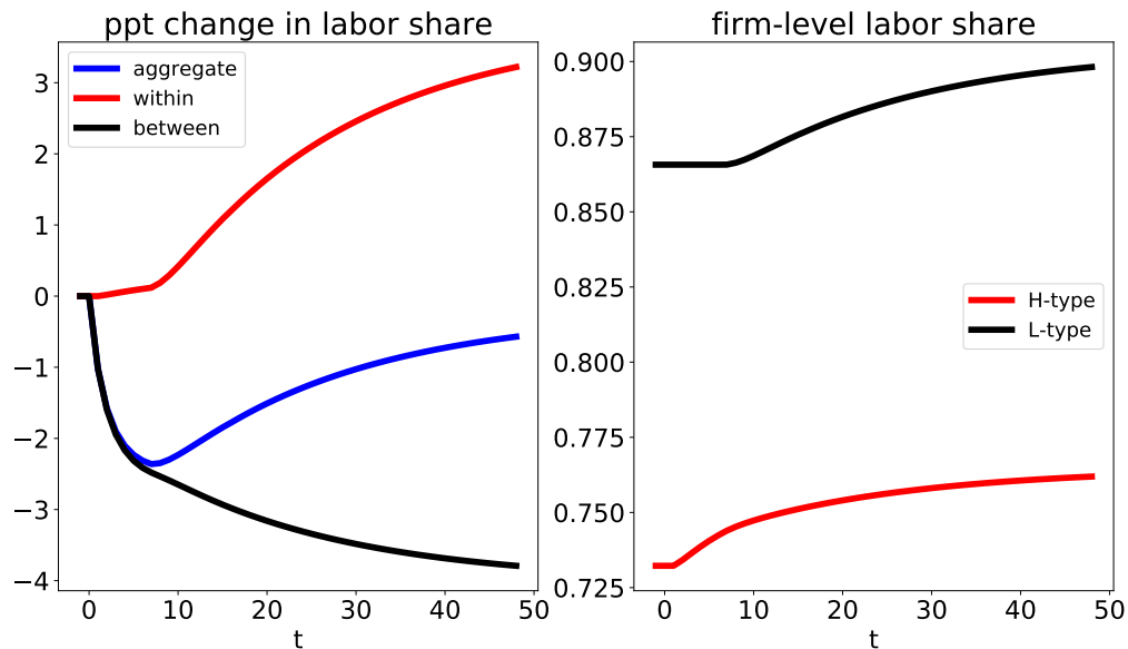
Figure 11: Labor share along the transition
