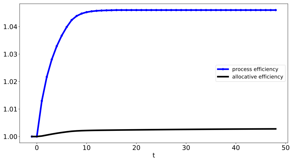
Figure 12: Process and allocative efficiency along the transition
