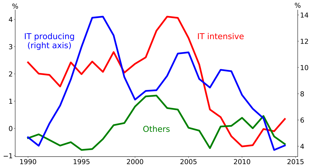
Figure 5: Productivity growth by IT intensity
