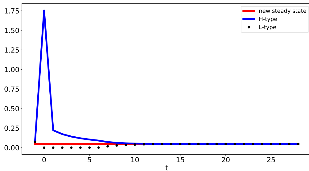
Figure 9: Transition dynamics of x/n
