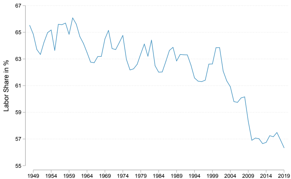
Figure A.1: U.S. labor share
