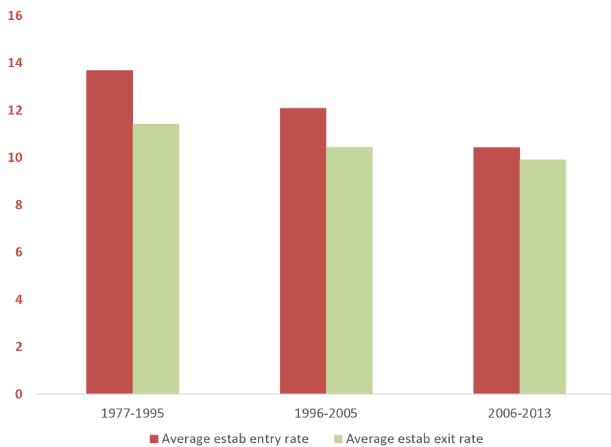
Figure A.3: Entry and exit rates of establishments
