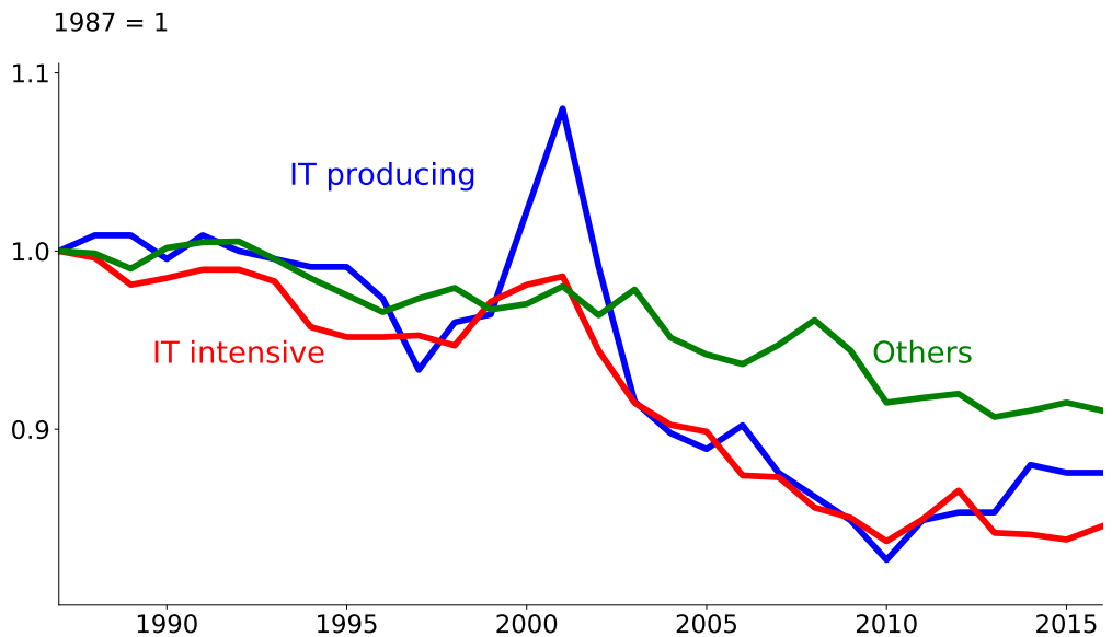
Figure 6: Labor share by IT intensity
