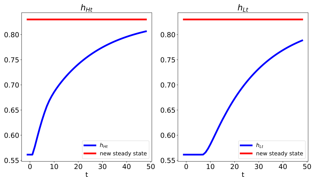
Figure 10: Transition dynamics of h_t
