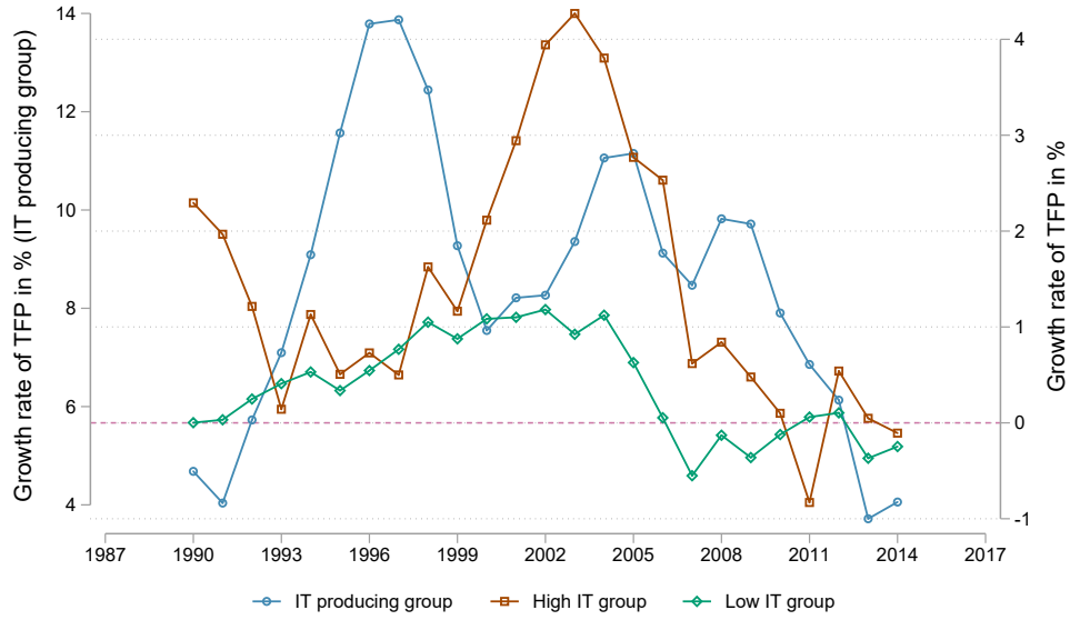
Figure E.1: Productivity growth by IT intensity - Alternative 1
