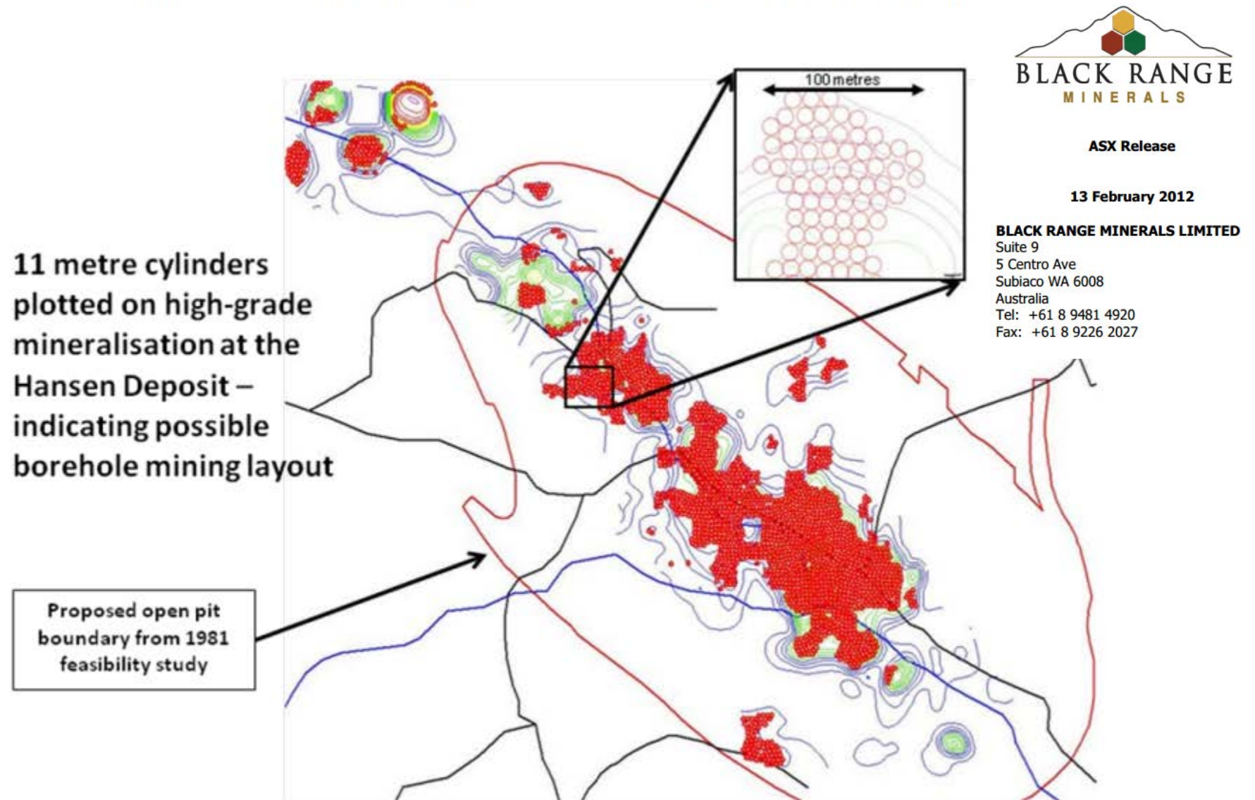
Figure 1. Possible Borehole Mining Layout at the Hansen Uranium Deposit – selectively targeting thicker and higher grade portions of the Deposit.
