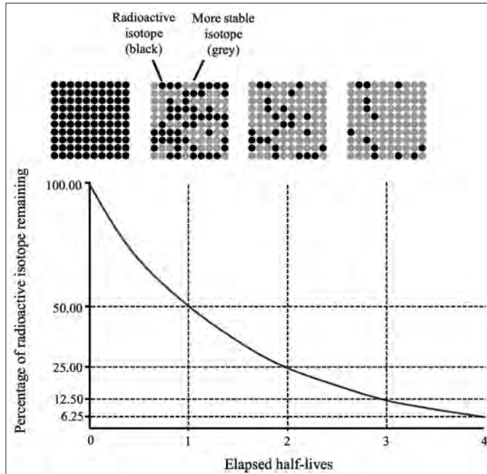
Fig. 1. Rate of decay of radioactive isotopes (image by Brent Nongbri, adapted from an image posted at https://tms Hughes.weebly.com/radioactive-decay-and-absolute-age-dating.html ).
