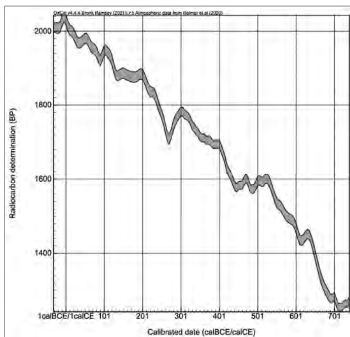
Fig. 2. A recent calibration curve for the first seven centuries CE showing radiocarbon years on the vertical axis and calendar years on the horizontal axis (image from OxCal v4.4.4, https://c14.arch.ox.ac.uk/oxcal/OxCal.html ).
