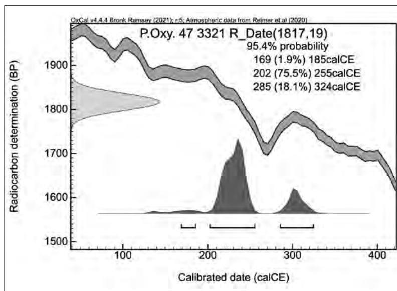
Fig. 8. Calibrated results for AMS analysis of P.Oxy. XLVII 3321 using OxCal v4.4.4.
